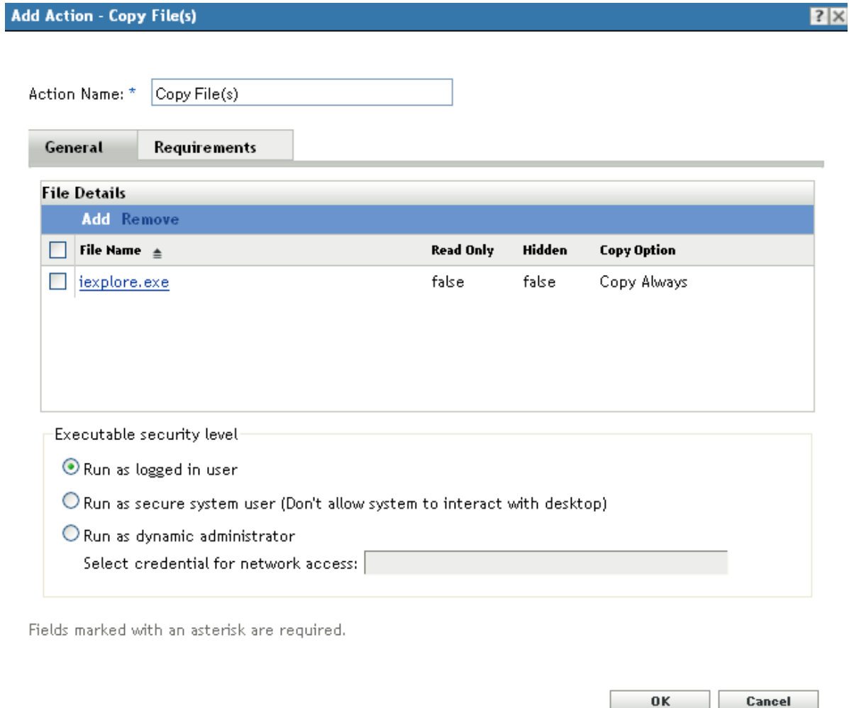
Figure 6-3 Action - Copy Files Dialog Box
